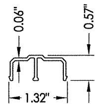
11 ROLLER TRACK
