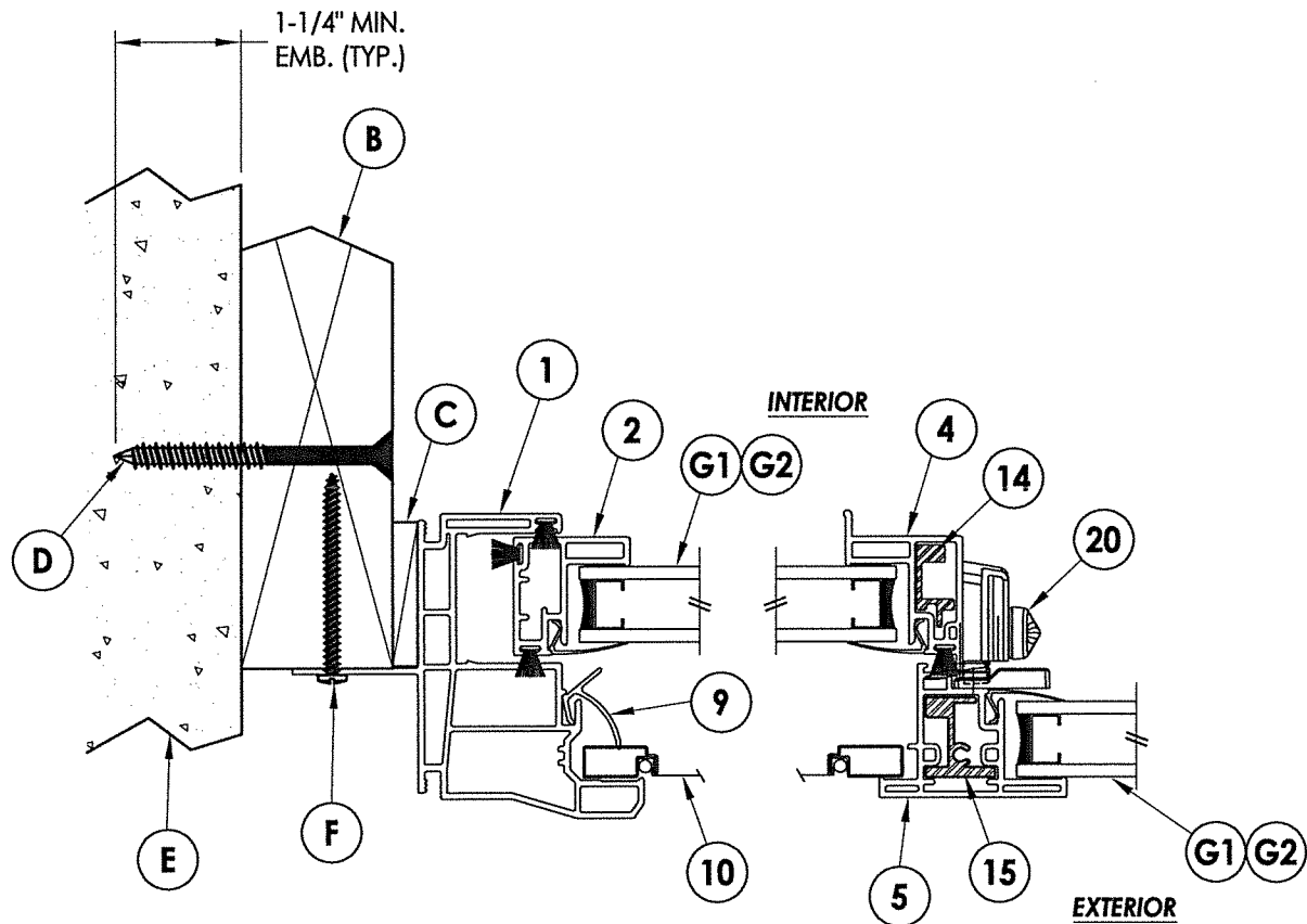
1 2 HORIZONTAL CROSS SECTION 2x Buck Construction
