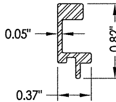
14 SASH STILE REINFORCEMENT
