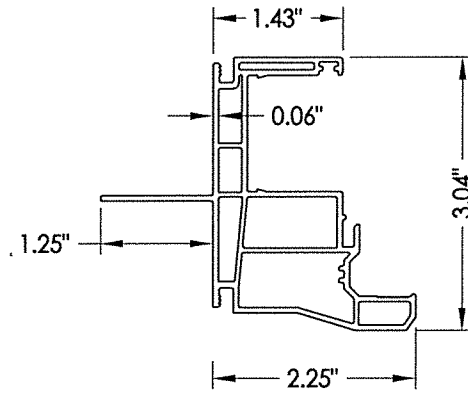
1 FRAME
