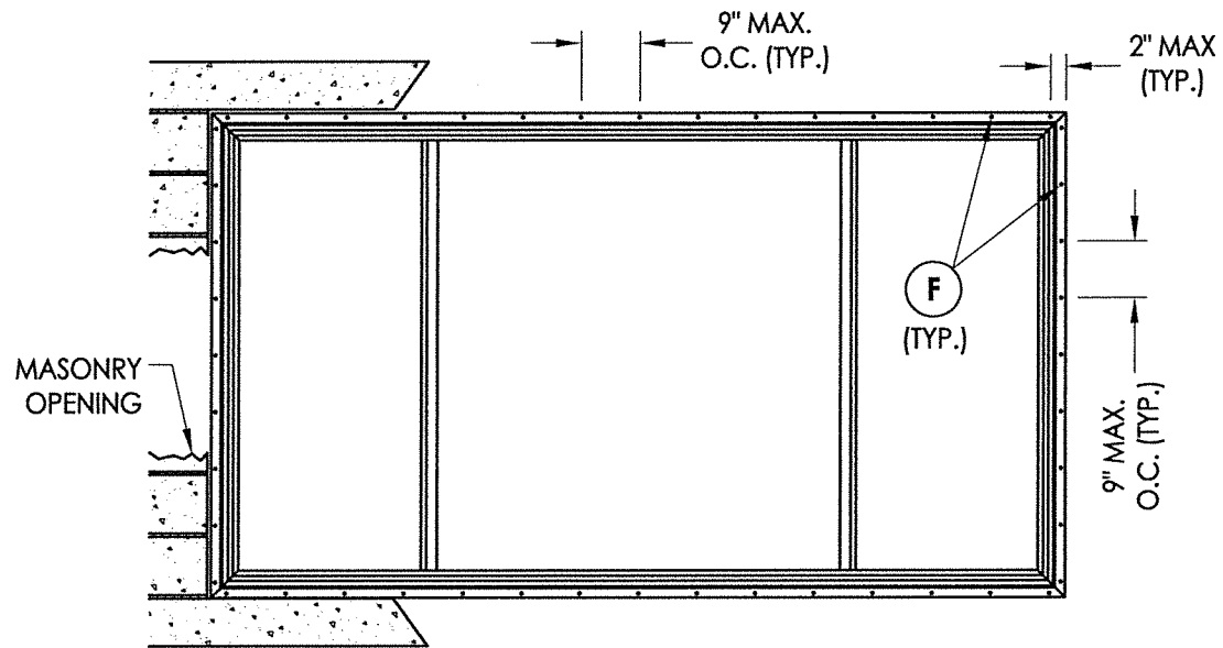
FRAME ANCHORING MASONRY CONSTRUCTION
