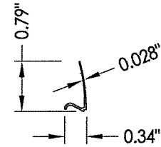
7 GLAZING BEAD
