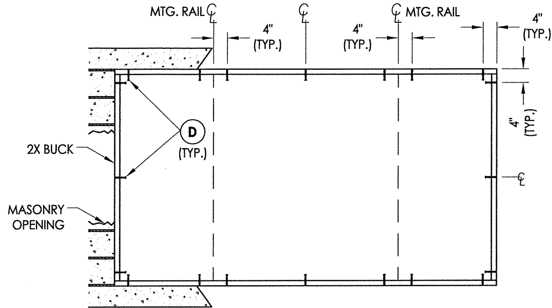
BUCK ANCHORING
