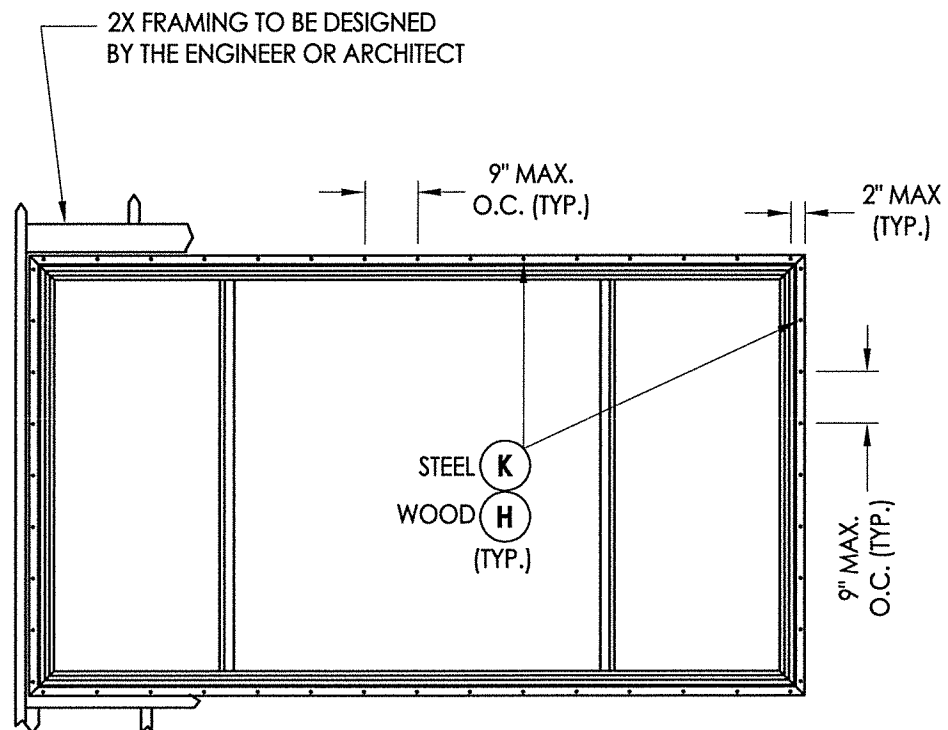
FRAME ANCHORING STUD CONSTRUCTION
