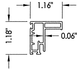
2 SASH STILE/RAIL
